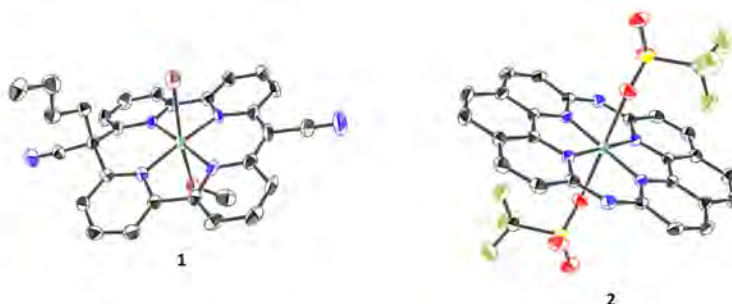
Figure 1) Single crystal structure of [\text{CoBr}(\text{butylpyr})\text{MeOH}] 1 and [\text{Co}(\text{OTf})_2(\text{azaphen})] 2 at 50% probability level; Hydrogen atoms were omitted for clarity; Black = Carbon, Blue = Nitrogen, Red = Oxygen, Green = \text{Co}^{2+} , Brown = Bromine, Yellow = Sulfur, Lime = Fluorine.
