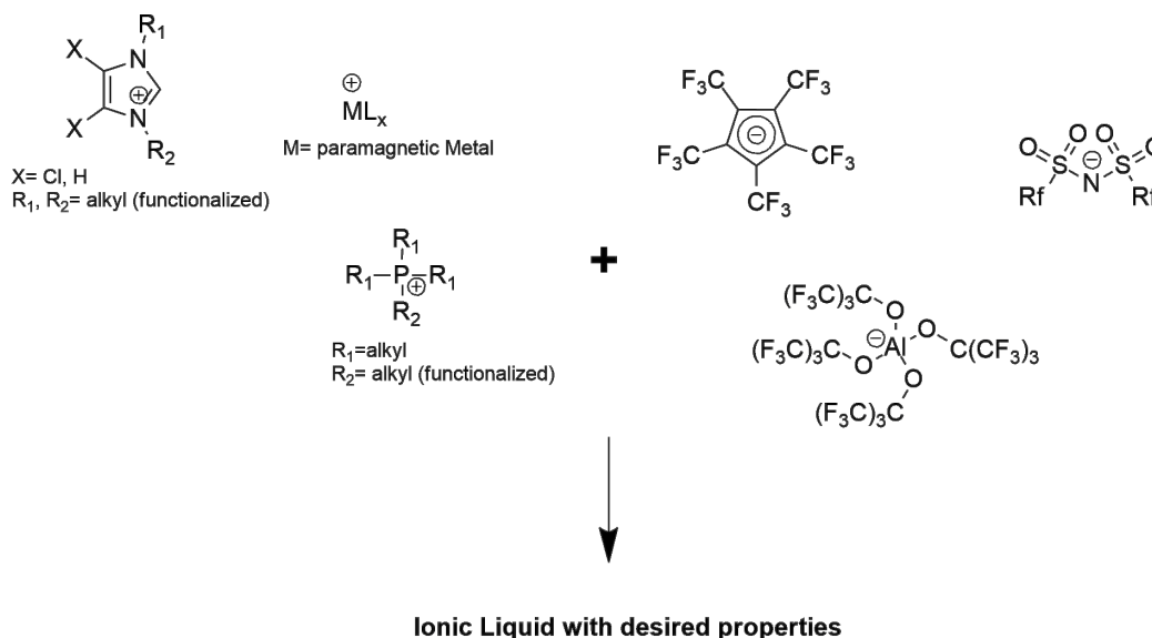
Scheme 1: Chemical construction kit for probe fillings.
