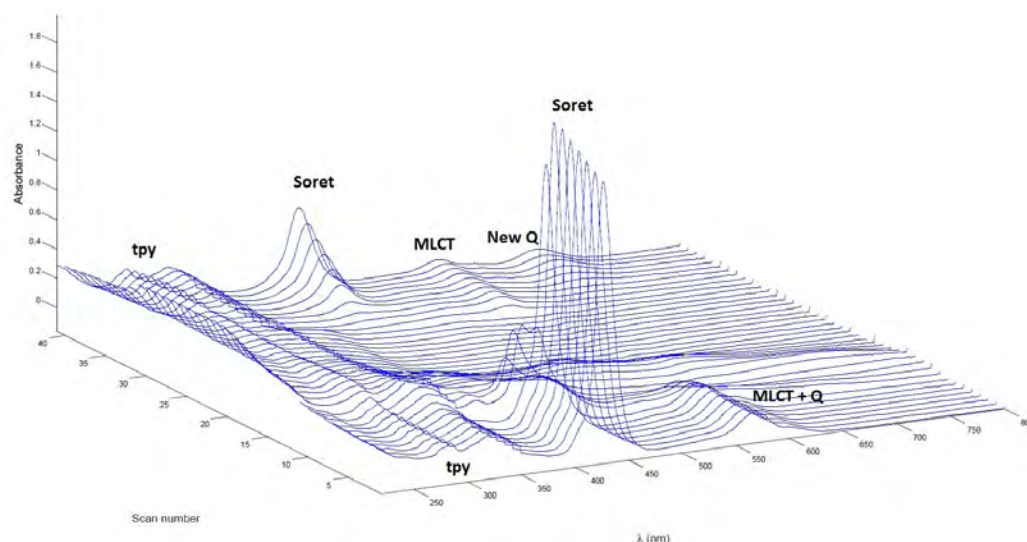
Figure: oxidative spectroelectrochemistry of the [Fe L 2 ] 2+ complex.
